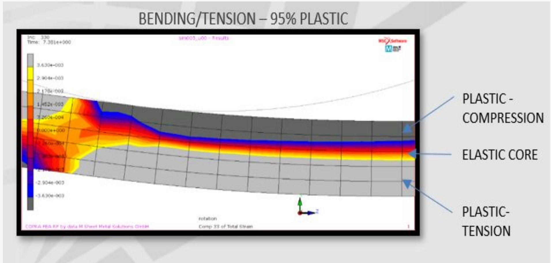
Roller Leveling Plasticity
