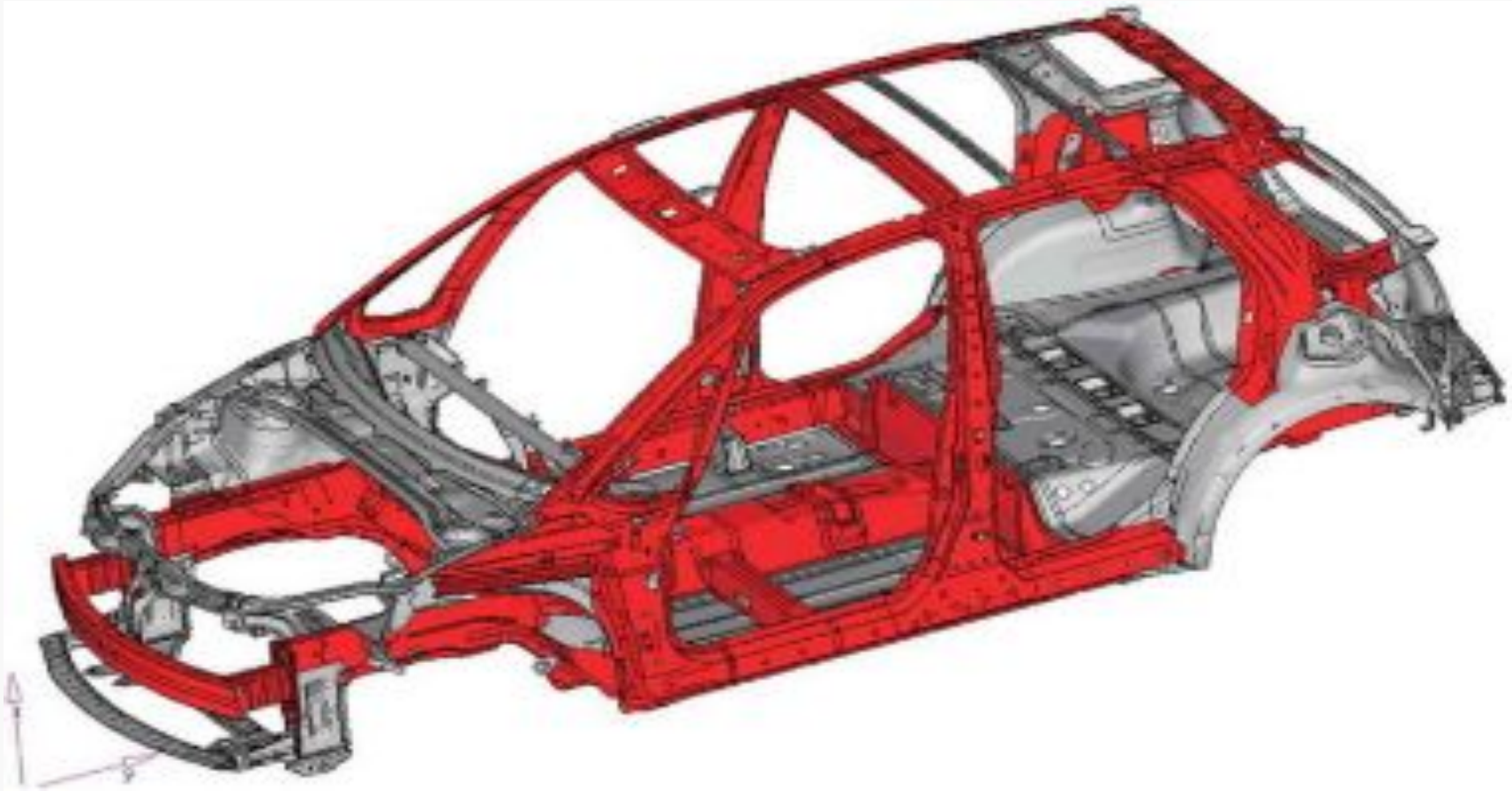
Example of areas using 3 rd Gen AHSS
