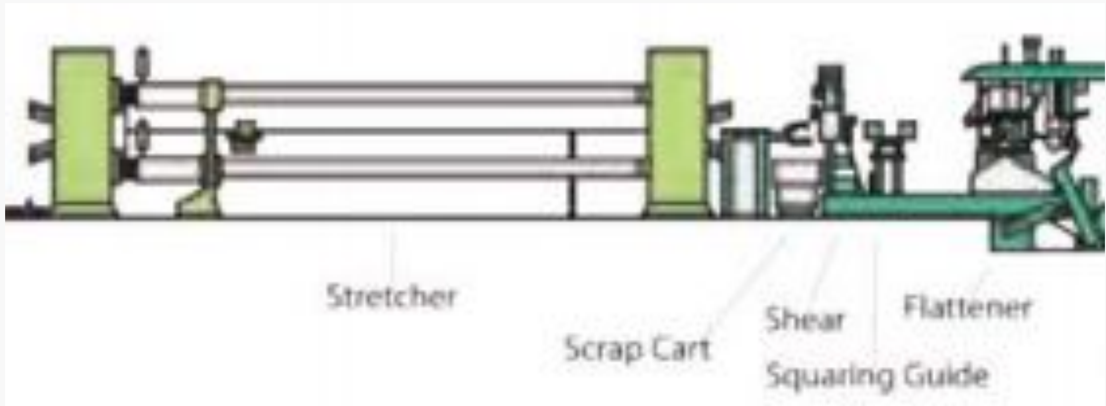
Simple illustration Stretcher Leveler
